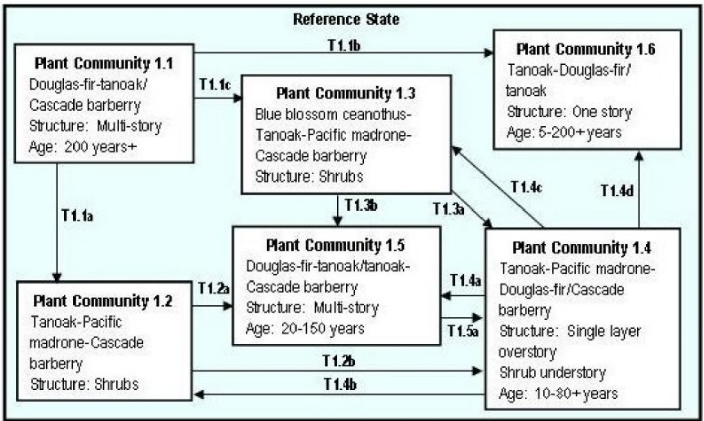
Figure 4. Douglas-fir-tanoak model
