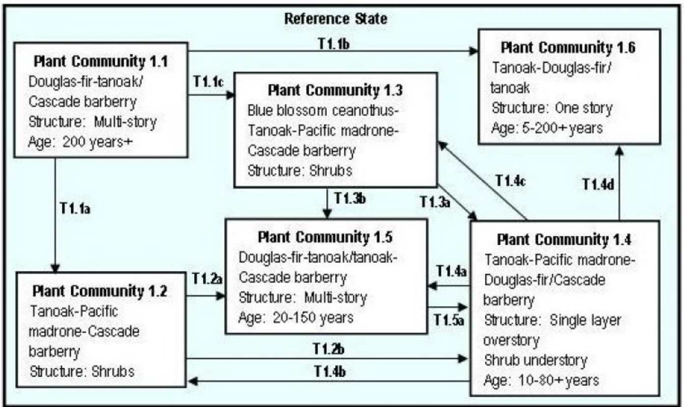
Figure 4. Douglas-fir-tanoak model
