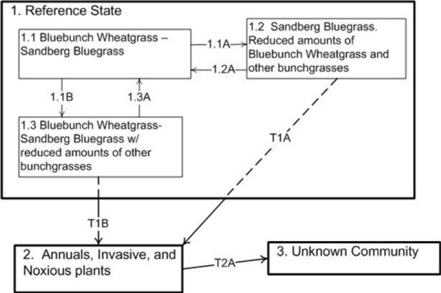
Figure 3. R008XY004ID
