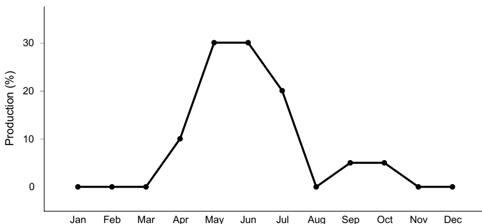
Figure 6. Plant community growth curve (percent production by month). ID0113, POPR/ARLU. State 2.
