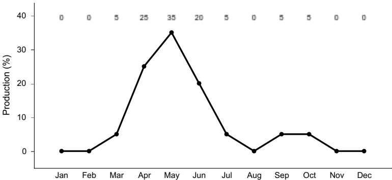
Figure 8. Plant community growth curve (percent production by month). ID0310, ARARL/FEID/ PSSPS. State 1.
