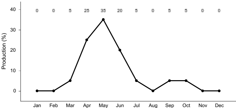
Figure 7. Plant community growth curve (percent production by month). ID0310, ARARL/FEID/ PSSPS. State 1.
