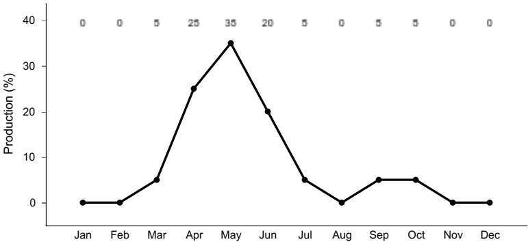
Figure 6. Plant community growth curve (percent production by month). ID0310, ARARL/FEID/ PSSPS. State 1.
