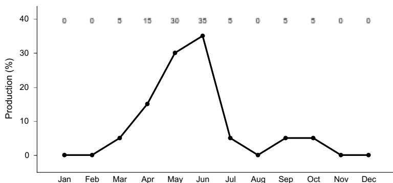
Figure 6. Plant community growth curve (percent production by month). OR4242, B10 JD Droughty Shallow South 9-12 B. State B: Disturbance .
