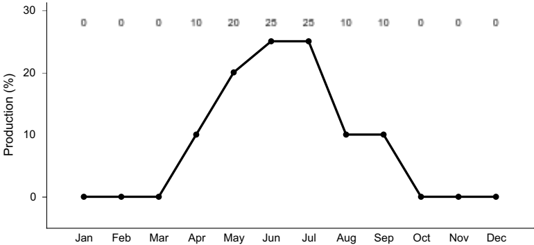
Figure 3. Plant community growth curve (percent production by month). ID0615, DRY MEADOW. State 2.
