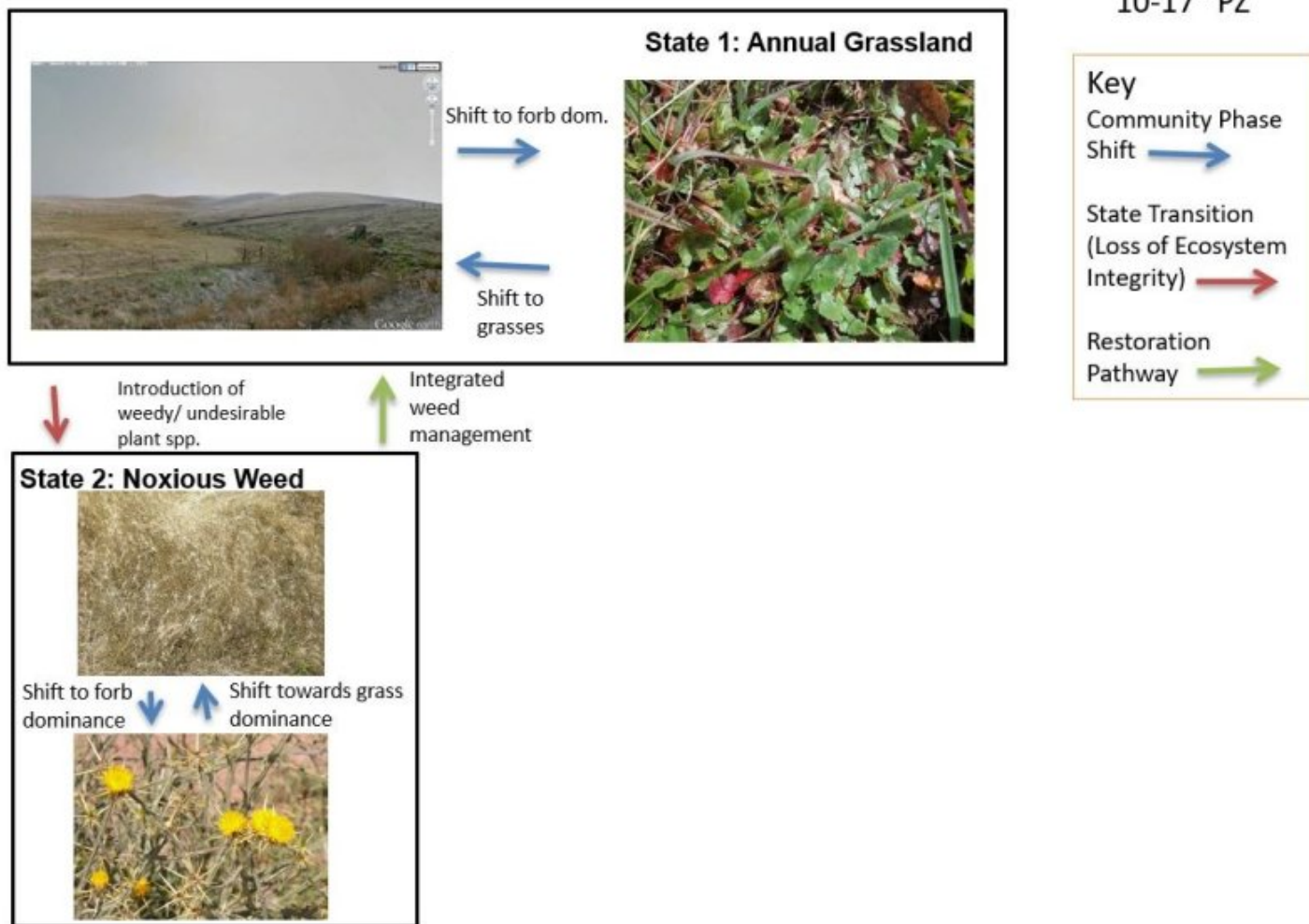
Figure 9. STM Photos
