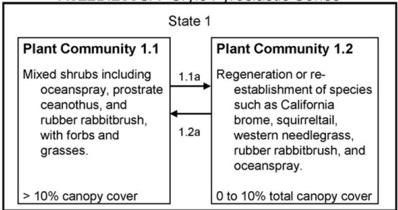
Figure 3. Cryic Pyroclastic Cone Model
