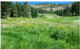
Hydrothermally Altered Seep Complex
