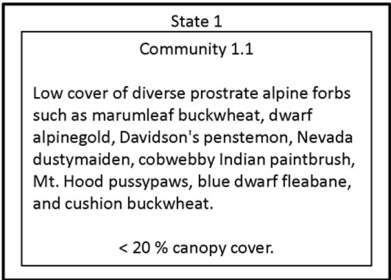
Figure 3. Pyroclastic Flow Model
