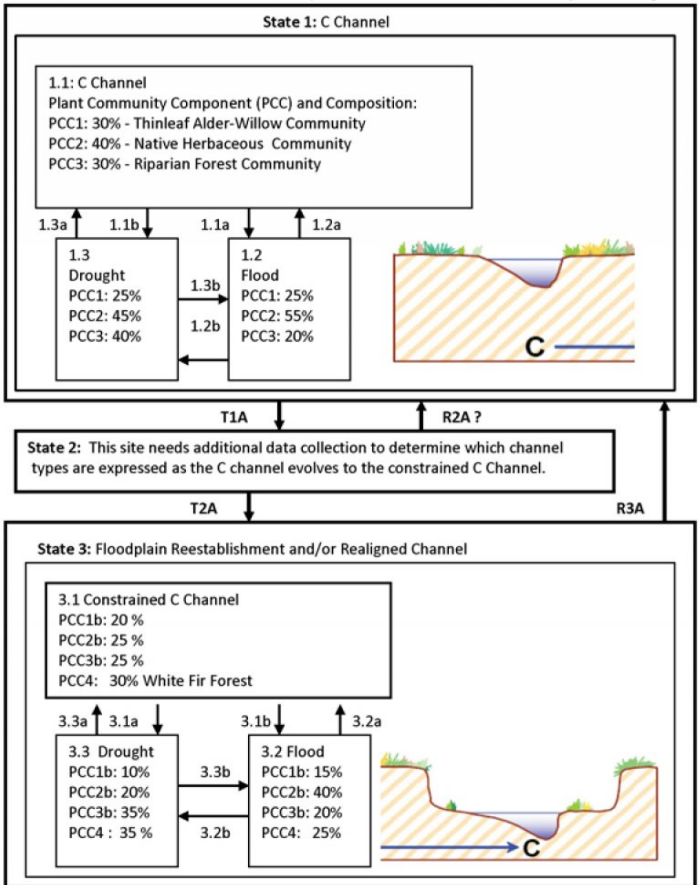
Figure 3. Frigid Gravelly Flood Plains Model
