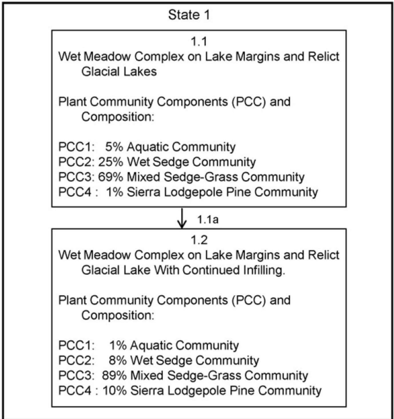
Figure 2. Frigid Lacustrine Flat Model
