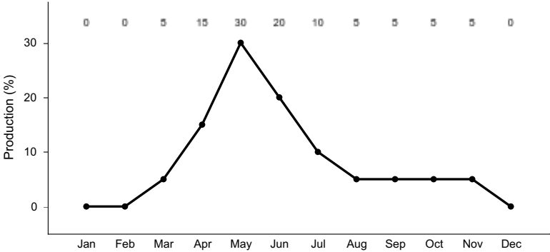
Figure 6. Plant community growth curve (percent production by month). ID0903, D25 JUOC/POSE/ANNUALS.
