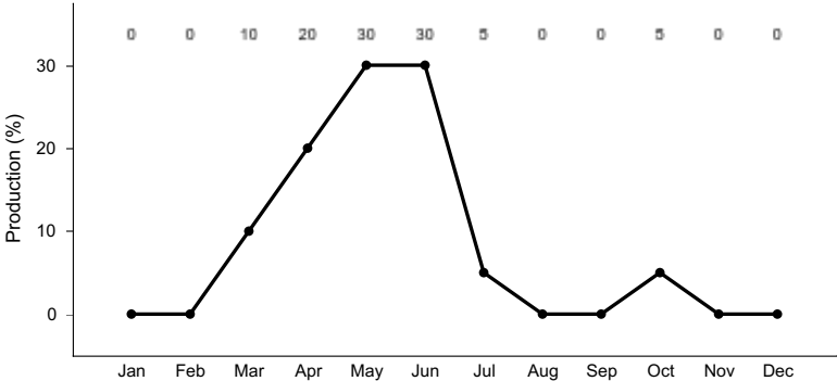
Figure 7. Plant community growth curve (percent production by month). ID0904, ARTRW8/PSSPS/ACTH7 HIGH PRECIP.
