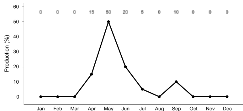
Figure 10. Plant community growth curve (percent production by month). WY0501, 5-9BH Upland sites. Monthly percentages of total annual growth for all upland sites with dominantly C3 Cool season plants..
