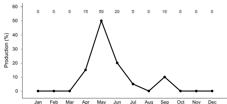
Figure 11. Plant community growth curve (percent production by month). WY0501, 5-9BH Upland sites. Monthly percentages of total annual growth for all upland sites with dominantly C3 Cool season plants..
