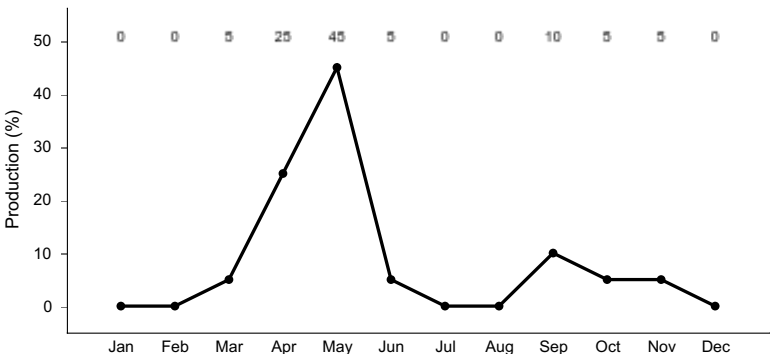
Figure 25. Plant community growth curve (percent production by month). WY0505, 5-9 BH Upland Sites, Annual Grasses Dominate. Monthly percentages of total annual growth, based on plant communities being affected by annual grasses (cheatgrass) or similar weedy species..
