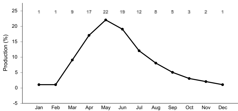
Figure 6. Plant community growth curve (percent production by month). UT0002, Current Potential. Community Phase 2.1.
