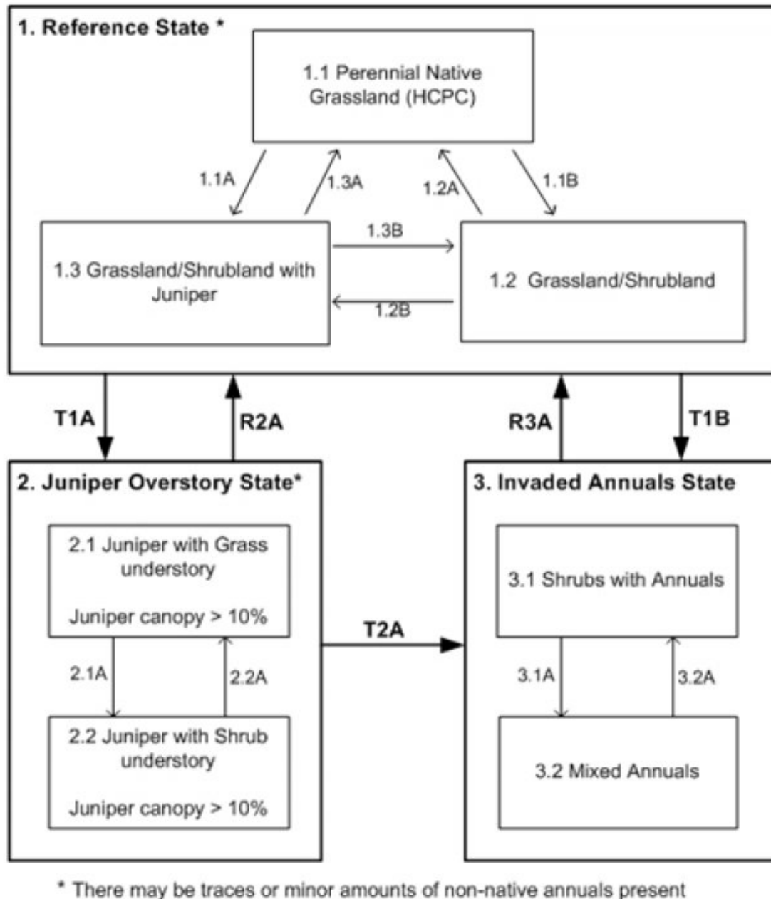
Figure 4. State and Transition - R035XA113AZ
