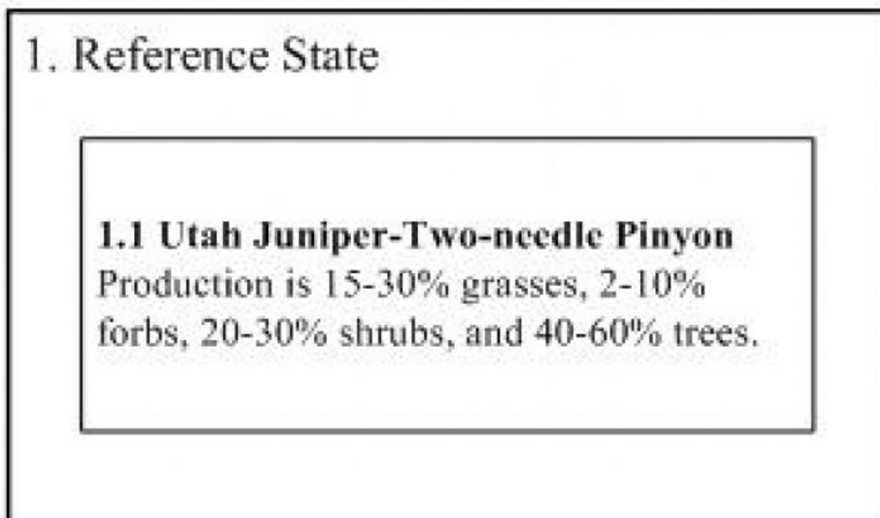
Figure 4. State-and-Transition Model
