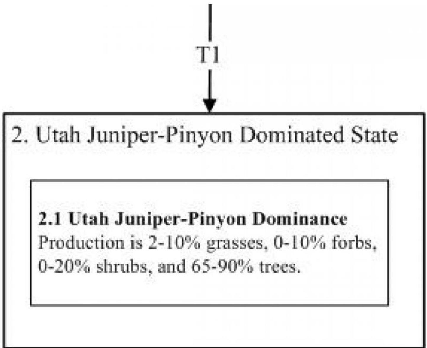
Figure 4. State-and-Transition Model
