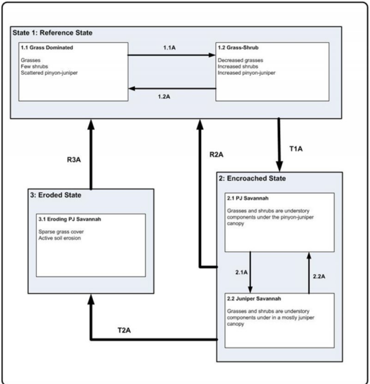
Figure 6. STM
