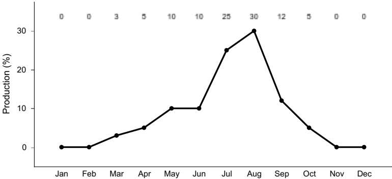
Figure 6. Plant community growth curve (percent production by month). NM0009, R036XB009NM Salt Meadow HCPC. R036XB009NM Salt Meadow HCPC Grassland with minor forb and shrub components..
