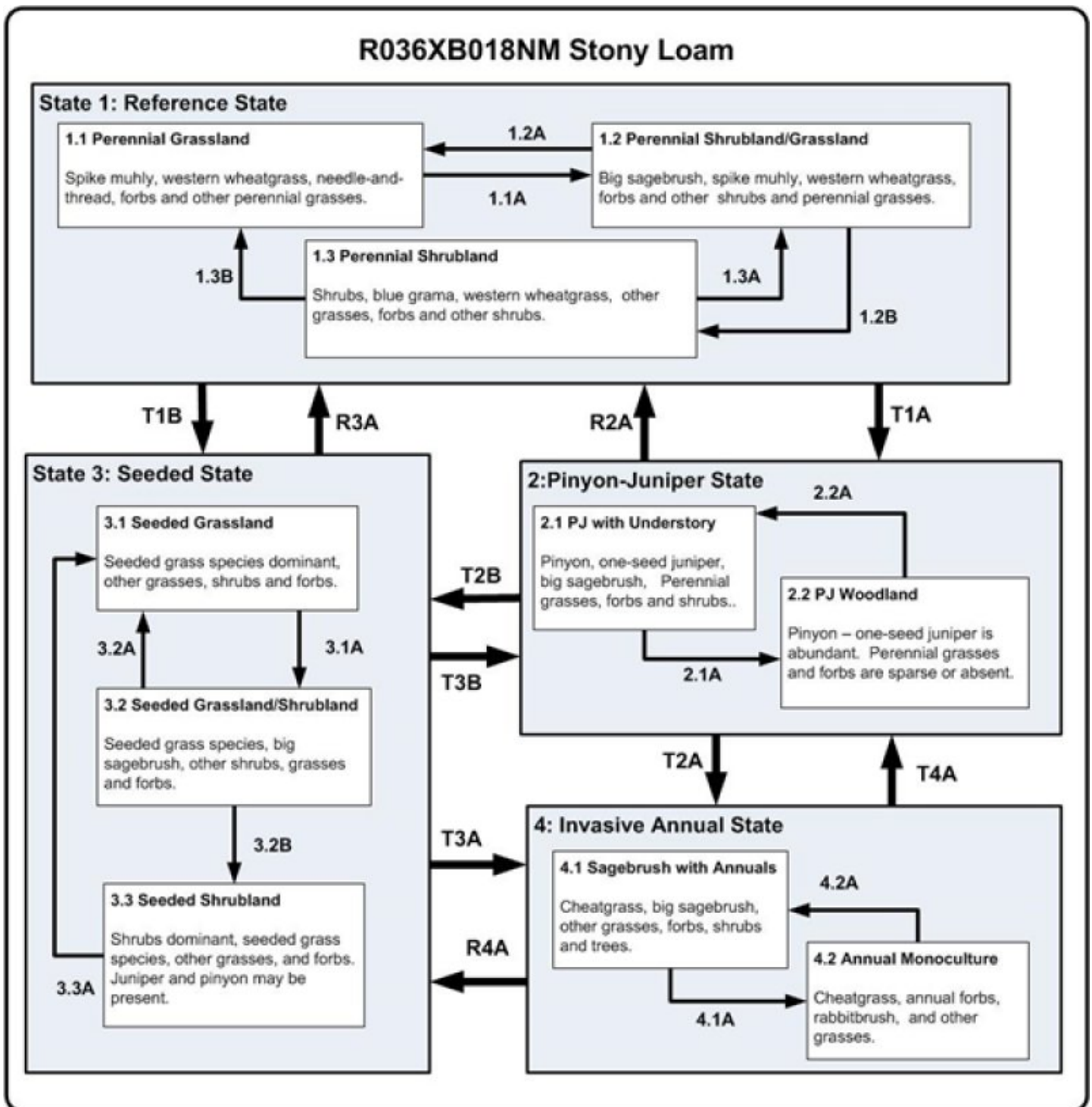
Figure 6. STM
