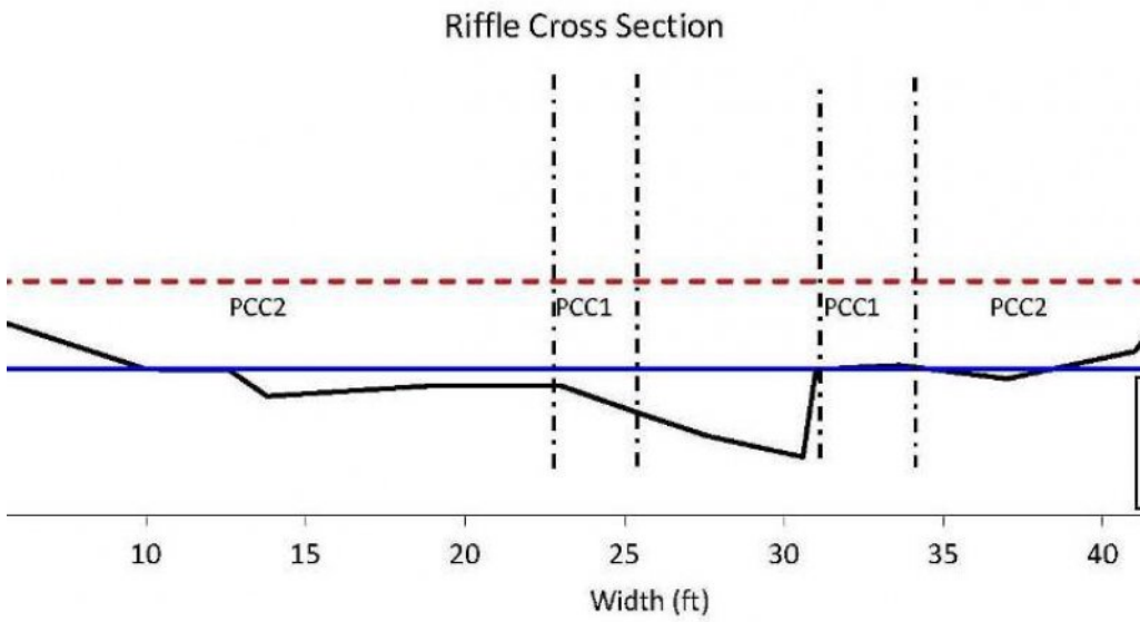
Figure 10. Stream channel cross section with PCC delineated.
