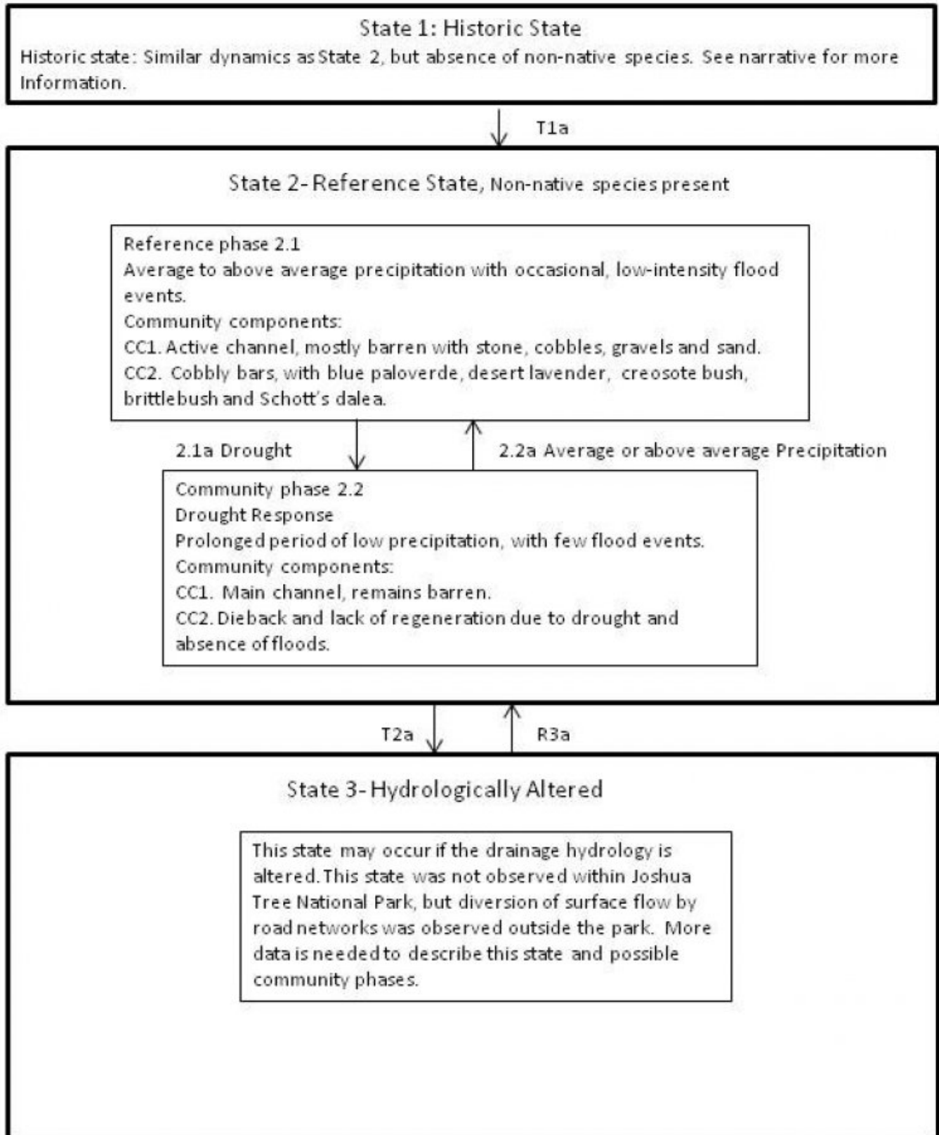
Figure 6. R031XY201CA Model
