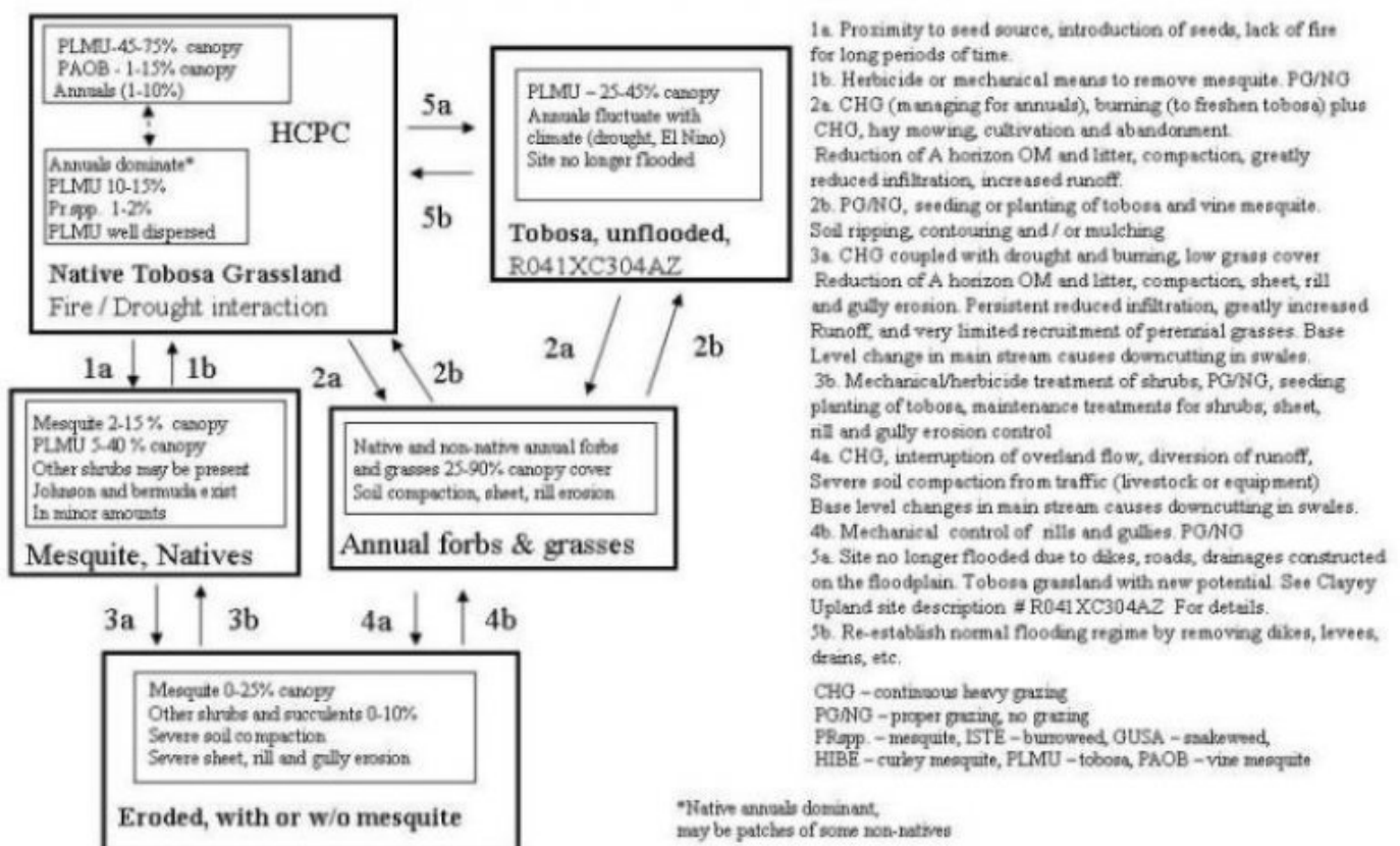
Figure 4. State and transition, Clayey Swale 12-16" p.z.
