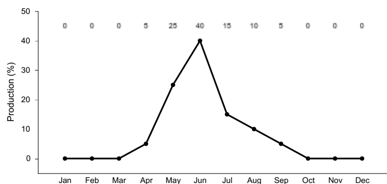
Figure 4. Plant community growth curve (percent production by month). MT0431, 43A - Uplands. Includes all upland sites in 43A.
