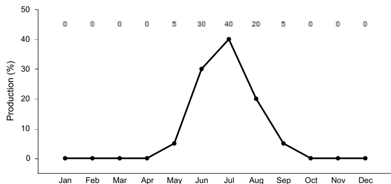
Figure 3. Plant community growth curve (percent production by month). WY0101, 20+ upland sites.
