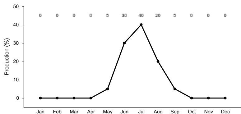
Figure 4. Plant community growth curve (percent production by month). WY0101, 20+ upland sites.
