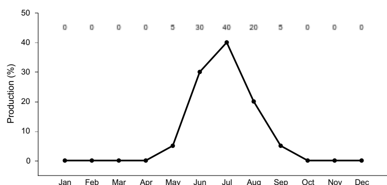
Figure 5. Plant community growth curve (percent production by month). WY0101, 20+ upland sites.
