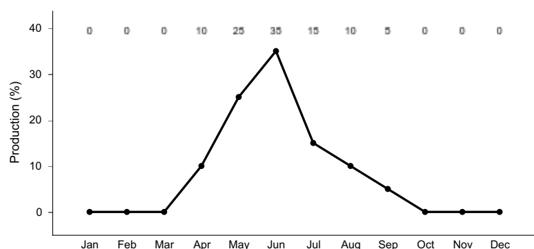
Figure 5. Plant community growth curve (percent production by month). MT0441, 44A - Uplands. Includes all upland sites in 44A.
