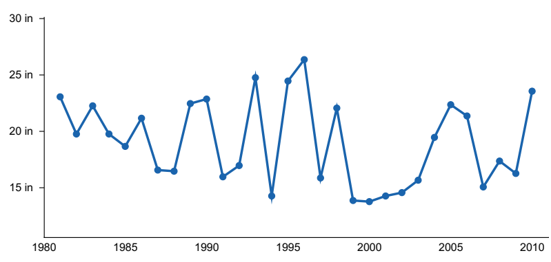
Figure 6. Annual precipitation pattern
