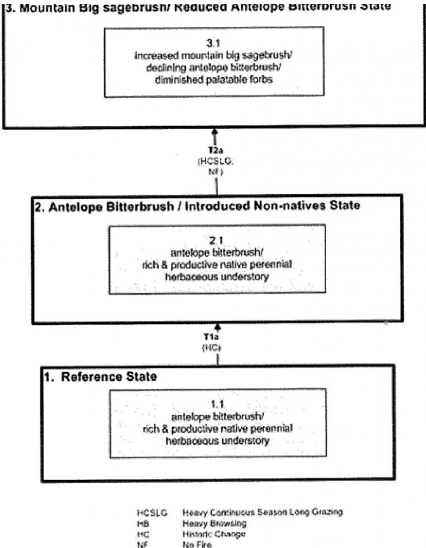
Figure 2. STM
