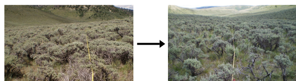
Sagebrush Dominant
