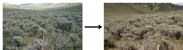
Bunchgrass Dominant
