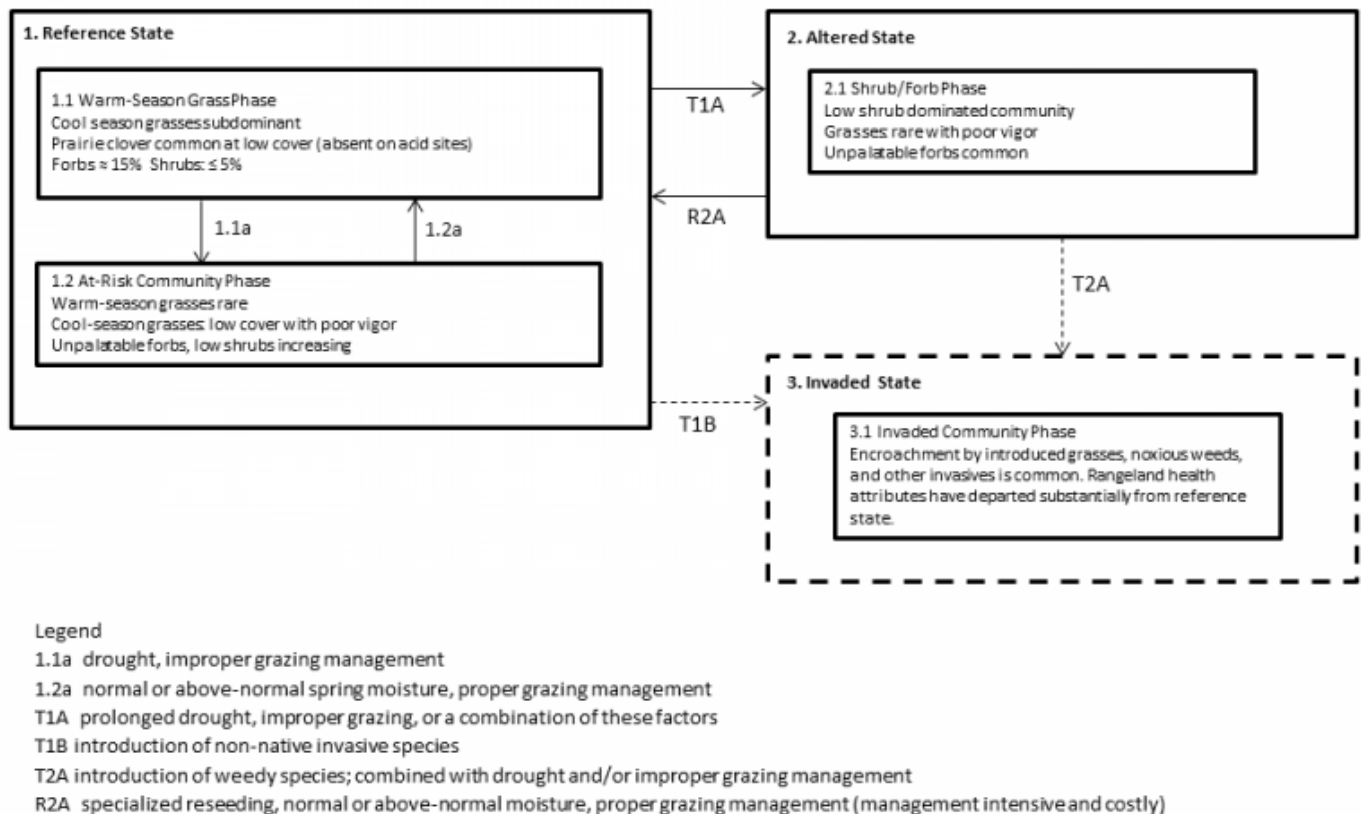
Figure 2. State-and-transition diagram
