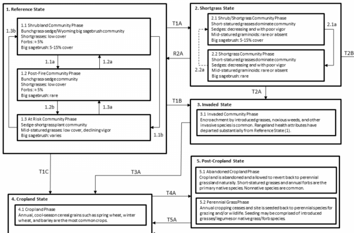
Figure 2. State-and-transition diagram.
