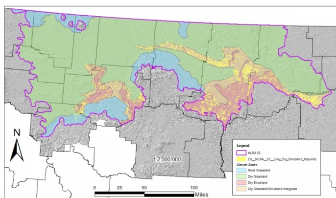
Figure 2. Figure 1. General distribution of the Limy Dry Shrubland ecological site by map unit extent.
