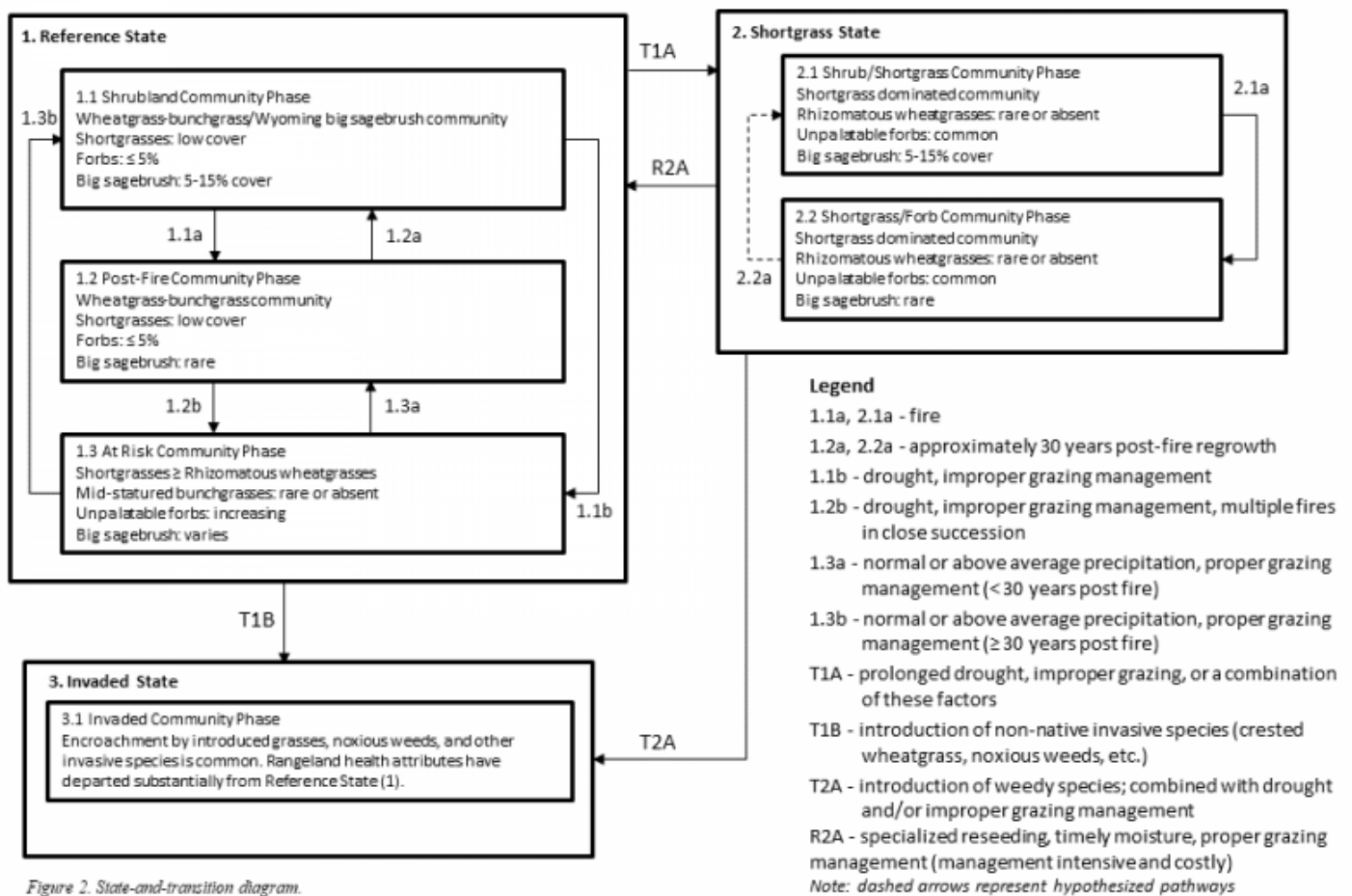
Figure 2. State-and-transition diagram.
