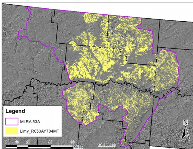
Figure 2. General distribution of the Limy ecological site by map unit extent.
