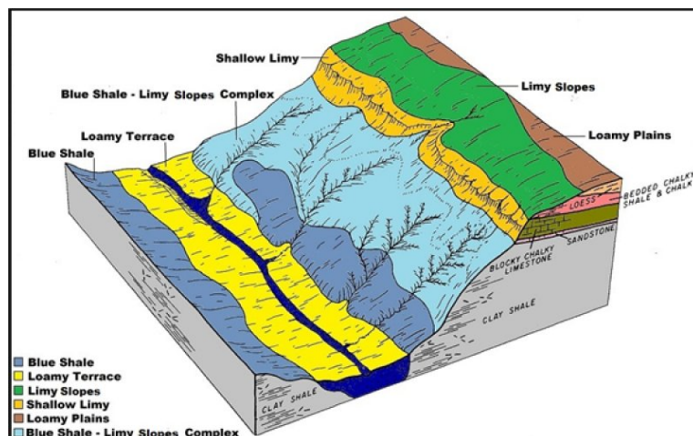
Figure 2. MLRA 73 ecological site block diagram.
