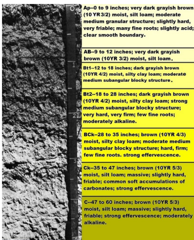
Figure 8. Harney soil profile, Ellis county Kansas.
