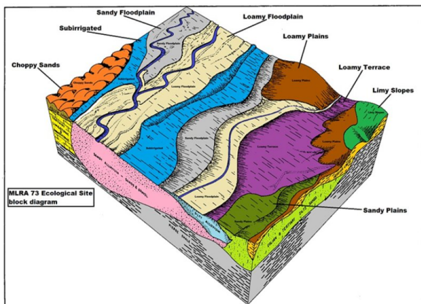
Figure 2. MLRA 73 Ecological Site block diagram.
