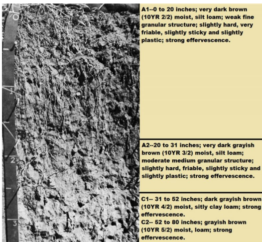
Figure 8. Roxbury soil series Ellis County, KS.
