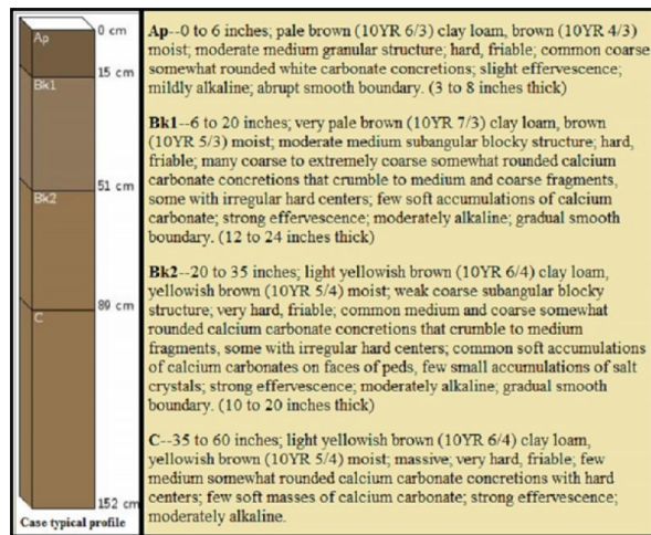
Figure 8. Case typical soil profile image.
