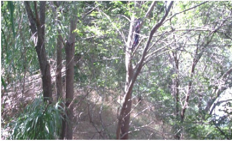
Figure 18. 2.2 Hardwood/Woodland Community
