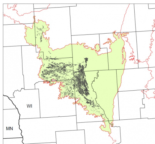
Figure 1. Distribution of Moist Siliceous Sand Uplands in the Wisconsin Central Sands MLRA (89).
