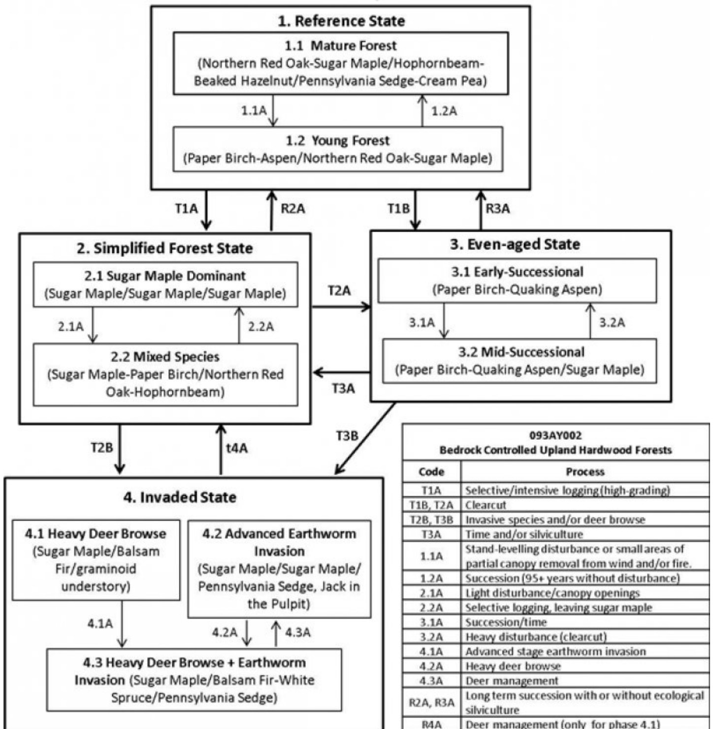
Figure 6. State-and-transition model.
