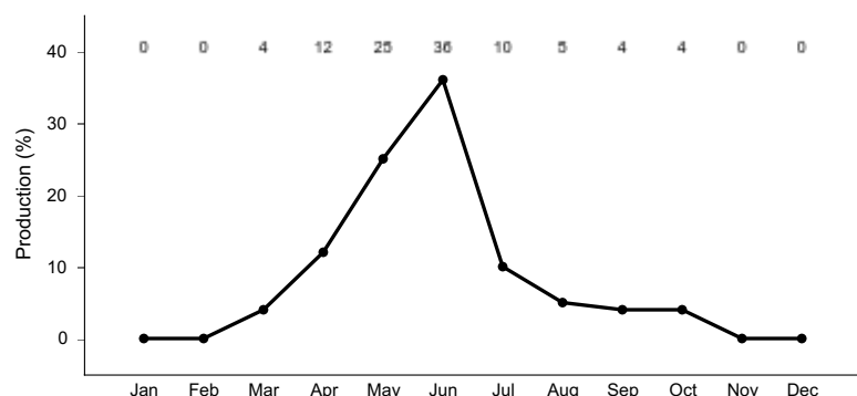
Figure 15. Plant community growth curve (percent production by month). SD0201, Rolling Till Prairie, cool-season dominant.. Cool-season dominant..
