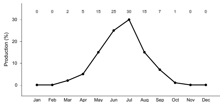
Figure 9. Plant community growth curve (percent production by month). SD0205, Rolling Till Prairie, warm-season dominant.. Warm-season dominant..
