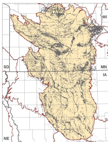
Figure 2. Distribution of the Sandy Upland Prairies ecological site within MLRA 103. In many cases, the data set is not spatially consistent across political boundaries due to the method by which soils were mapped; e.g. due to county subsets.
