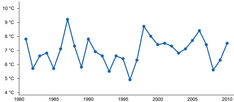
Figure 8. Annual average temperature pattern
