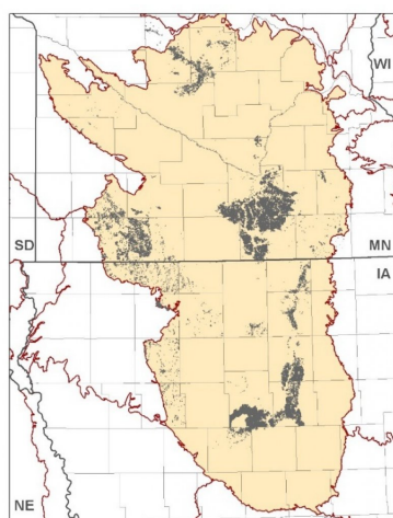
Figure 2. Distribution of Clayey Wet Prairies within MLRA 103. In many cases, data is not spatially consistent across political boundaries due to the method with which soils were mapped; e. g. county subsets.
