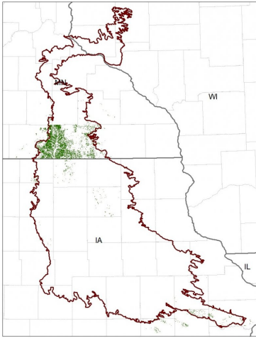
Figure 2. Figure 1. Location of Wet Loamy Upland Savanna ecological site within MLRA 104.
