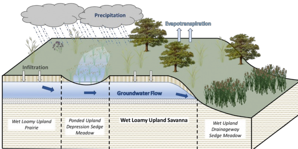
Figure 9. Figure 4. Hydrologic cycling in Wet Loamy Upland Savanna ecological site.
