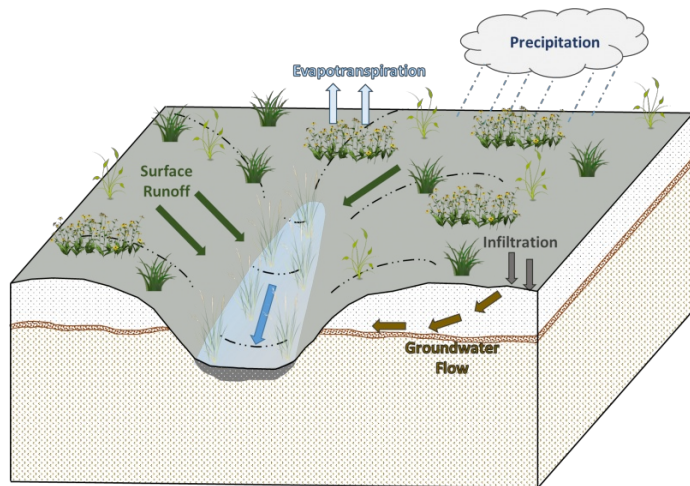
Figure 10. Figure 5. Hydrologic cycling in Wet Upland Drainageway Sedge Meadow ecological site.
