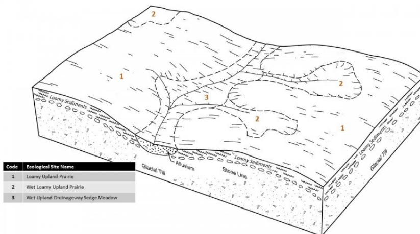
Figure 3. Figure 2. Representative block diagram of Wet Upland Drainageway Sedge Meadow and associated ecological sites.
